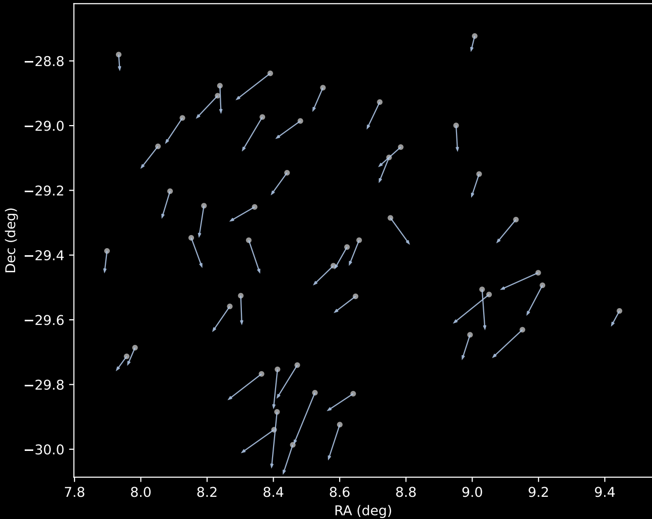
APOGEE DR17 Cluster 1 Proper Motion Vectors (n=48)
