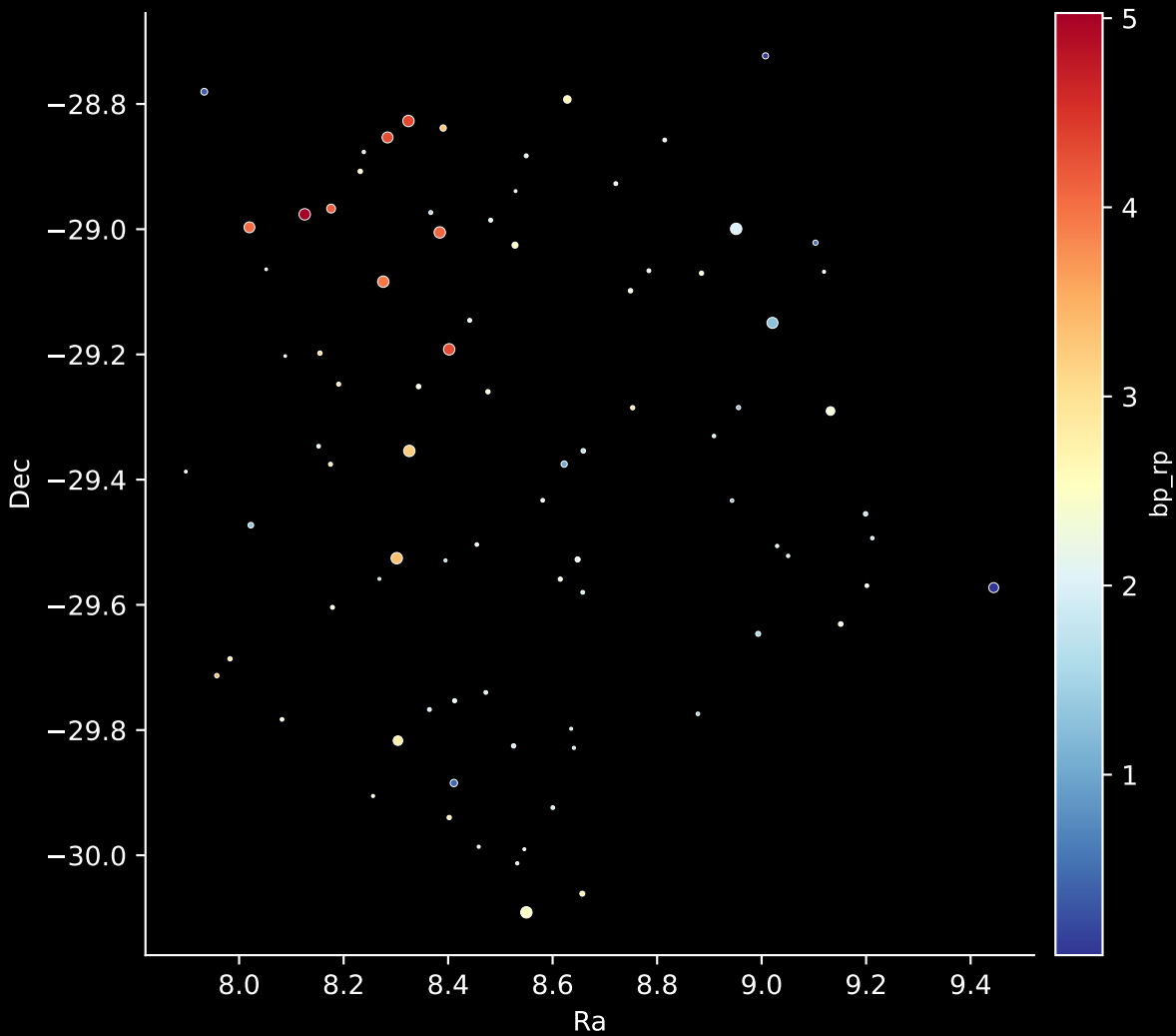
APOGEE DR17 Field: [001-02-O] Stars: 84
