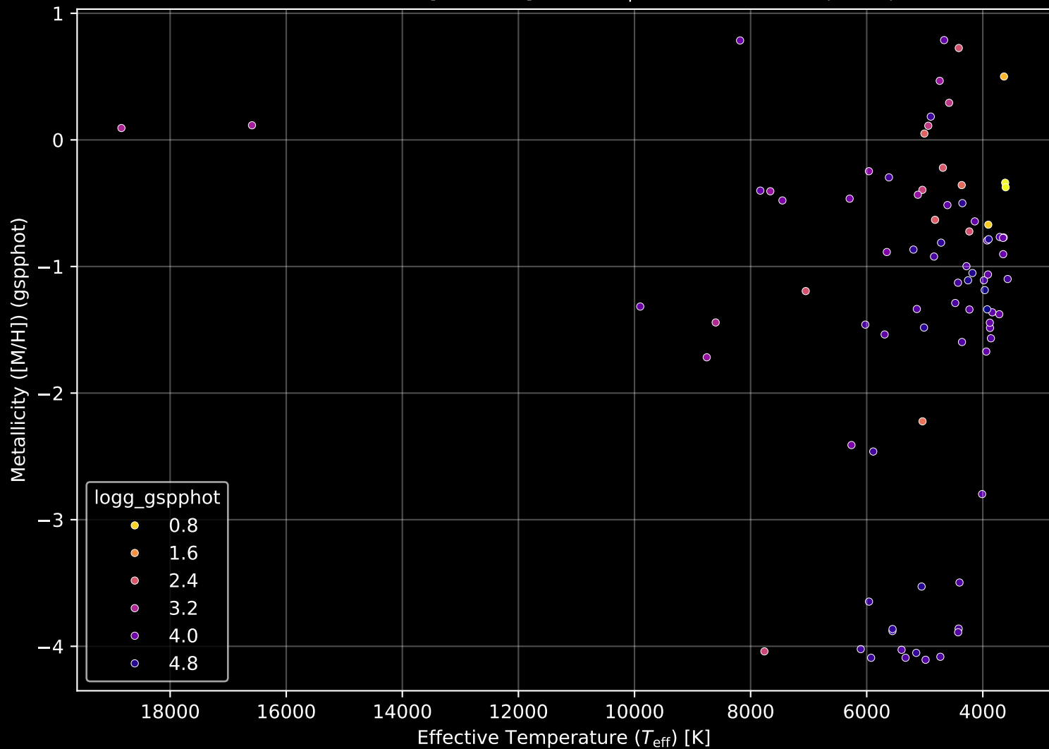
APOGEE DR17 Field: [001-02-O] Stellar Population Parameters (n= 84)
