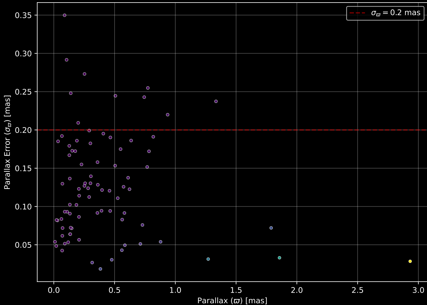
APOGEE DR17 Field: [001-02-O] Parallax Quality (n= 84)
