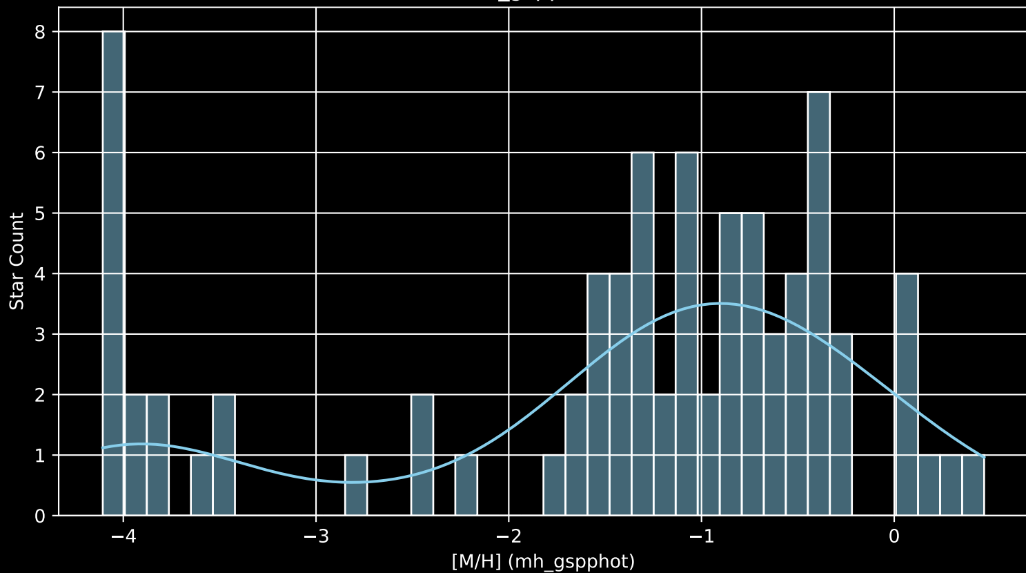
APOGEE DR17 Field: [001-02-O [M/H] (mh_gspphot) (n= 80)
