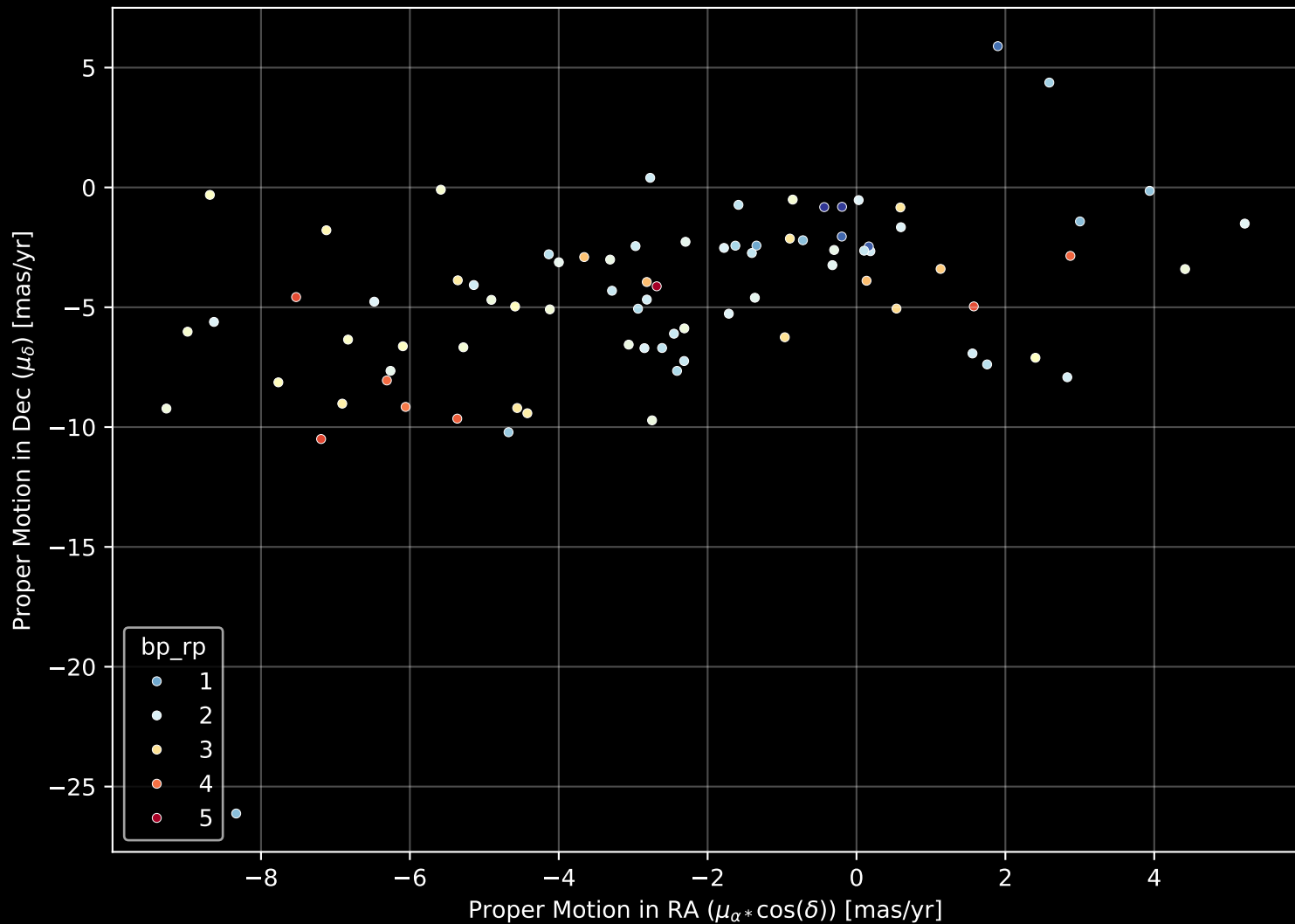
APOGEE DR17 Field: [001-02-O] Proper Motion Diagram (n= 84)
