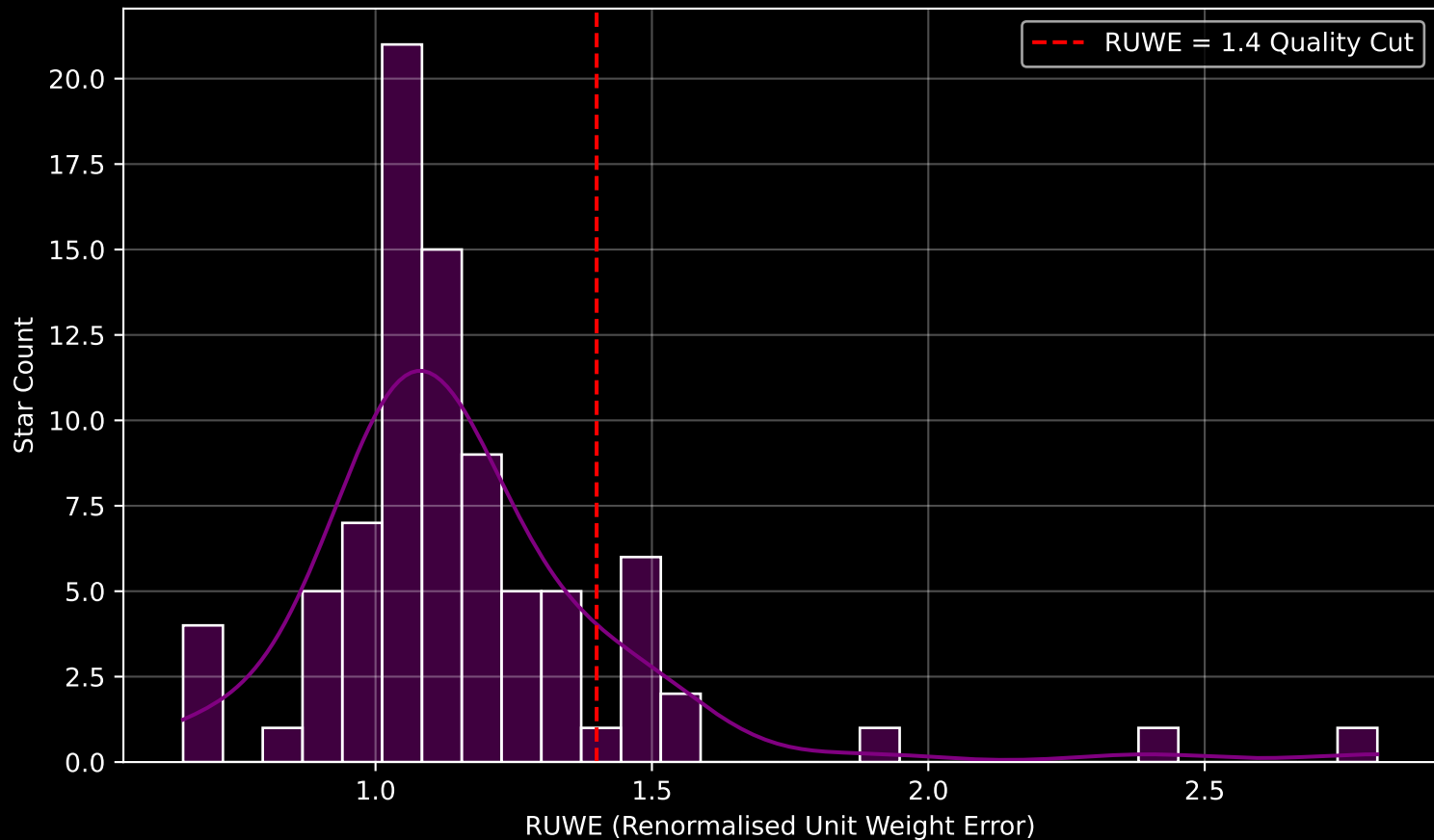
GAPOGEE DR17 Field [001-02-O] RUWE Distribution (n= 84)
