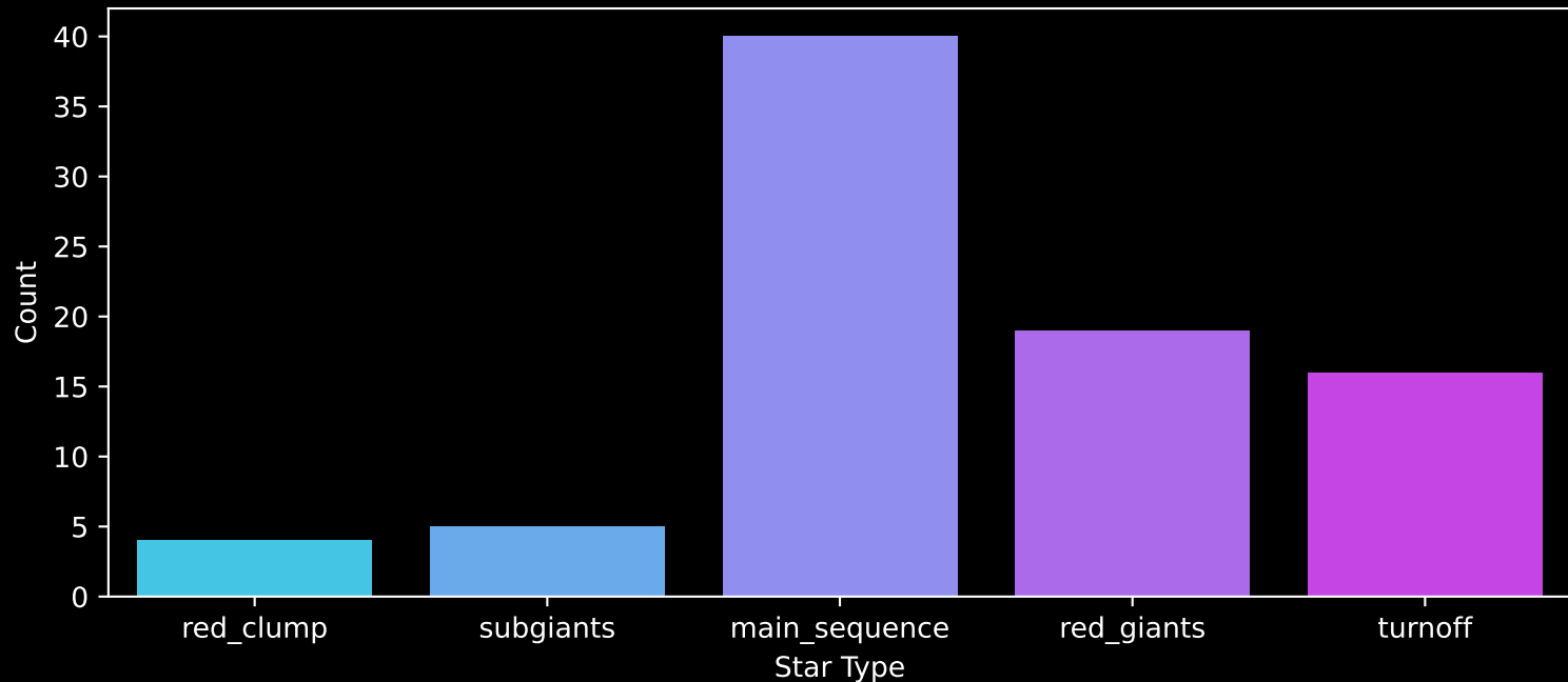
APOGEE DR17 Field: [001-02-O] Count plot of Star Type
